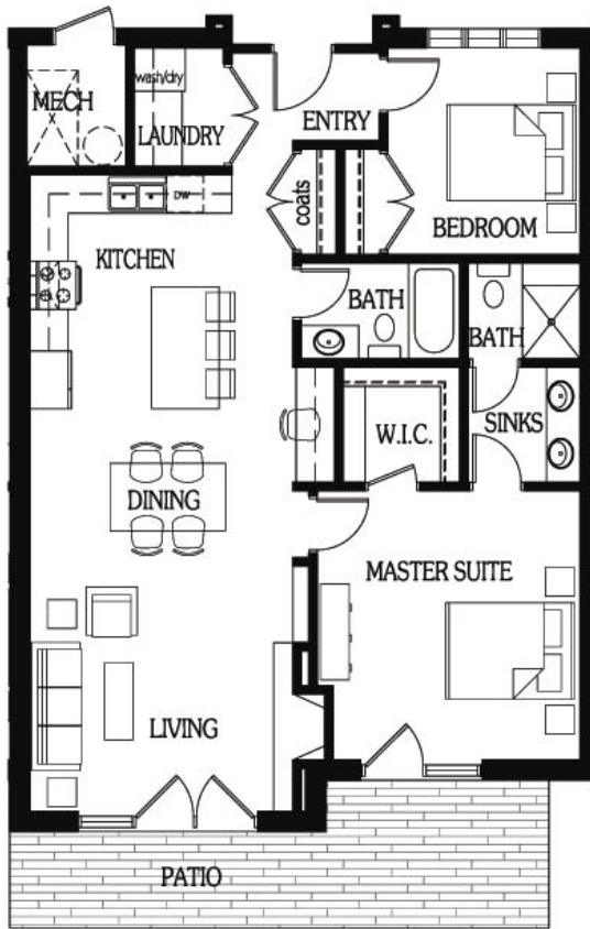
first floor unit two floor plan
